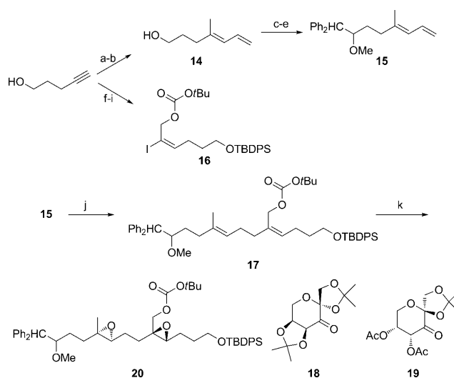
Scheme 3. Synthesis of the cascade cyclization substrate. Reagents and conditions: a) Me 3 Al, Cp 2 ZrCl 2 , H 2 O, DCE, then I 2 , 94 %; b) CH 2 =CHMgBr, [Pd(PPh 3 ) 4 ], PhMe, 91 %; c) Oxalyl chloride, DMSO, CH 2 Cl 2 , Et 3 N, -78 °C; d) Ph 2 CH 2 , n BuLi, THF, 82 % (two steps); e) NaH, DMF, then MeI, 96 %; f) TBDPSCl, imidazole, DMF, 100 %; g) n BuLi, THF, then (CH 2 O) n , 94 %; h) Bu 3 SnH, [Pd(PPh 3 ) 4 ], C 6 H 6 , then I 2 , CH 2 Cl 2 , 83 %; i) (Boc) 2 O, N -methylimidazole, PhMe, 99 %; j) 9-BBN dimer, THF, then 16 , [Pd(PtBu 3 ) 2 ], K 3 PO 4 , H 2 O, PhMe, 74 %; k) Oxone, 18 , K 2 CO 3 , Bu 4 NHSO 4 , CH 3 CN, H 2 O, then 19 , 82 %. 9-BBN = 9-borabicyclo [3.3.1] nonane, Boc = tert -butoxycarbonyl, DMF = N,N -dimethylformamide, DMSO = dimethyl sulfoxide, TBDPS = tert -butyldiphenylsilyl, THF = tetrahydrofuran.
