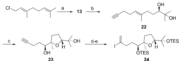
Scheme 5. Synthesis of the right-hand fragment. Reagents and conditions: a) 1-Trimethylsilylpropyne, n BuLi, THF, -78^\circ\text{C} , then \text{Bu}_4\text{NF} , 88%; b) AD-Mix \beta , \text{CH}_3\text{SO}_2\text{NH}_2 , t BuOH, \text{H}_2\text{O} , 53%; c) 18 , Oxone, \text{K}_2\text{CO}_3 , \text{Bu}_4\text{NHSO}_4 , \text{CH}_3\text{CN} , \text{H}_2\text{O} , then Py-CSA, 83%, d.r. = 13:1; d) TESCl, imidazole, DMAP, DMF, 89%; e) \text{Et}_3\text{SiH} , [\text{CpRu}(\text{NCCH}_3)_3]\text{PF}_6 , \text{CH}_2\text{Cl}_2 , then \text{I}_2 , 2,6-lutidine, 82%. Cp = cyclopentadienyl, DMAP = 4-dimethylaminopyridine, Py-CSA = pyridinium camphorsulfonate, TES = triethylsilyl.
