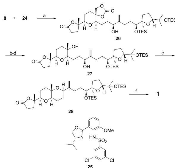
Scheme 6. Completion of the synthesis. Reagents and conditions: a) \text{CrCl}_2 , \text{NiCl}_2\cdot\text{DMP} , 25 , Proton Sponge, Mn, \text{Cp}_2\text{ZrCl}_2 , LiCl, \text{CH}_3\text{CN} , 84%, d.r. = 8:1; b) \text{K}_2\text{CO}_3 , MeOH, 91%; c) TsCl, \text{Et}_3\text{N} , \text{Bu}_2\text{SnO} , \text{CH}_2\text{Cl}_2 , 92%; d) \text{NaBH}_4 , HMPA, 50^\circ\text{C} , 76%; e) \text{Me}_3\text{P}=\text{C}(\text{H})\text{CN} , \text{C}_6\text{H}_6 , 80^\circ\text{C} , 40%; f) \text{Bu}_4\text{NF} , THF, 77%. DMP = 2,9-dimethylphenanthroline, HMPA = hexamethylphosphoramide.
