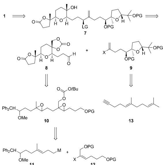
Scheme 2. Retrosynthesis of 1 . LG = leaving group, M = metal, PG = protecting group.
