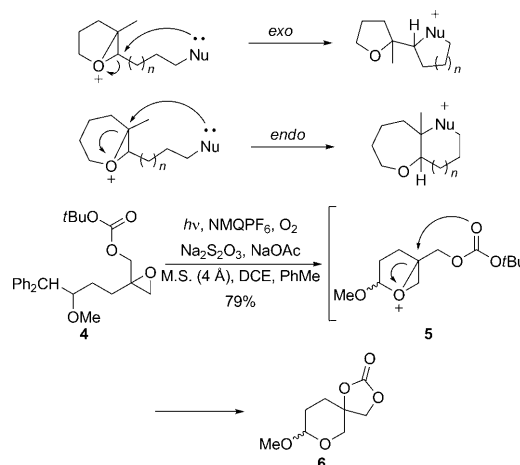
Scheme 1. Synthesis of oxygen-containing heterocycles through epoxonium-ion opening. DCE = 1,2-dichloroethane, M.S. = molecular sieves, NMQPF 6 = N -methylquinolinium hexafluorophosphate.
