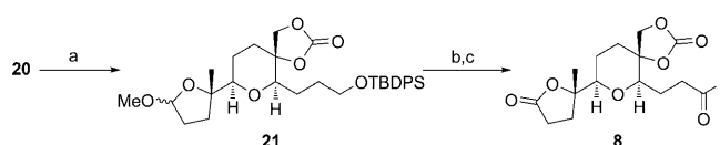
Scheme 4. Completion of the left-hand fragment. Reagents and conditions: a) hν , NMQPF 6 , O 2 , Na 2 S 2 O 3 , NaOAc, DCE, PhMe, 45 % yield of isolated product (75 % based on recovered starting material); b) m CPBA, Sc(OTf) 3 , CH 2 Cl 2 , 68 %; c) IBX, DMSO, 93 %. IBX = 2-iodoxybenzoic acid, m CPBA = meta -chloroperoxybenzoic acid, Tf = tri-fluoromethanesulfonyl.
