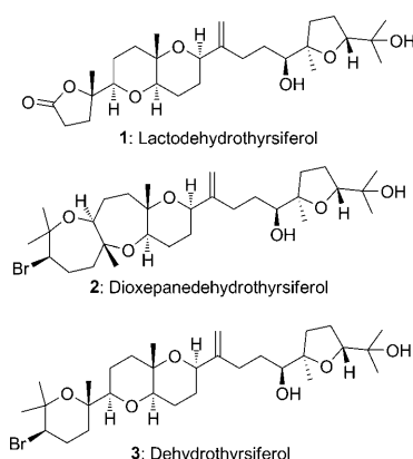
Figure 1. Squalene-derived ethers from red algae.
